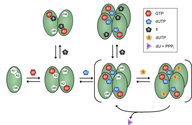
Figure 2. Double hit inhibition mechanism of 1 . Compound 1 intercepts the ordered-essential activation mechanism of SAMHD1 by binding to the A2 activator site in a nonproductive manner that cannot lead to tetramer formation ( K_i = 50 \mu\text{M} ). In addition, 1 binds to the catalytic site and competitively inhibits substrate binding. Binding of the GTP activator to the A1 site is required to assemble dimers and to form the A2 site. The scheme also depicts the previously determined mechanistic feature where SAMHD1 turns over without release of bound activator nucleotides (brackets).
